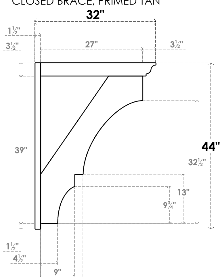
SIDE PROFILE
